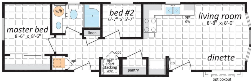
CB - 12422 12' x 42' • 504 sq. ft.
