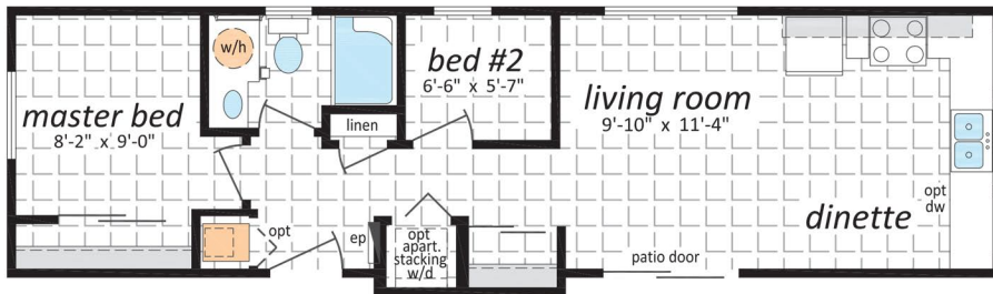
CB - 12443 12' x 44' • 528 sq. ft.
